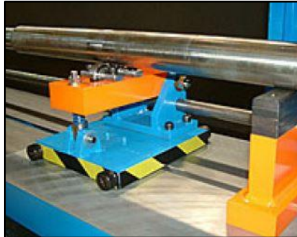
2. O.D. ROLLER SUPPORT
