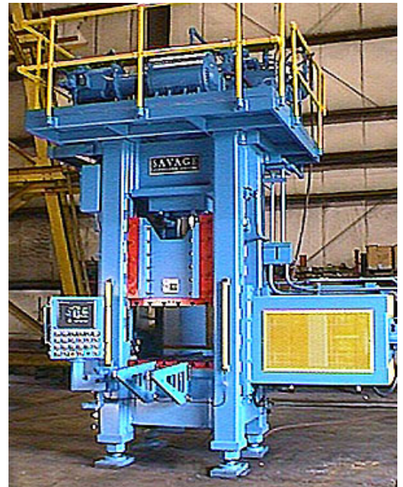
350 Ton Punch Press with barfeeder for 1 1/4" thick max. barstock.
