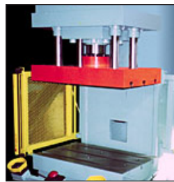
4-Post / 8-Bushing Guided Platen
